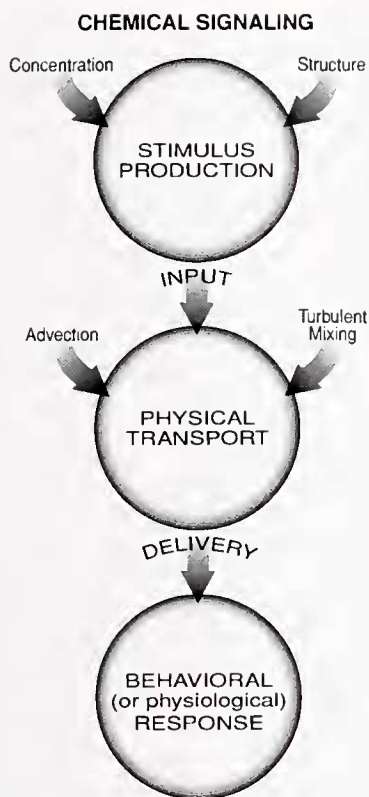
Figure 1. Diagram of the factors that determine the production, transport, and perception of waterborne chemical signals by a macroscopic organism.
